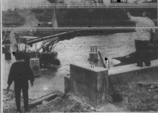
Construction supervisor Roy Elder directs his crew as work continues on a new bridge across the Medina River on Mayan Ranch Road Monday, Dec. 9. The next step, says Elder, is the forming and pouring of a 17-inch-thick concrete roadway that will span between the columns.
